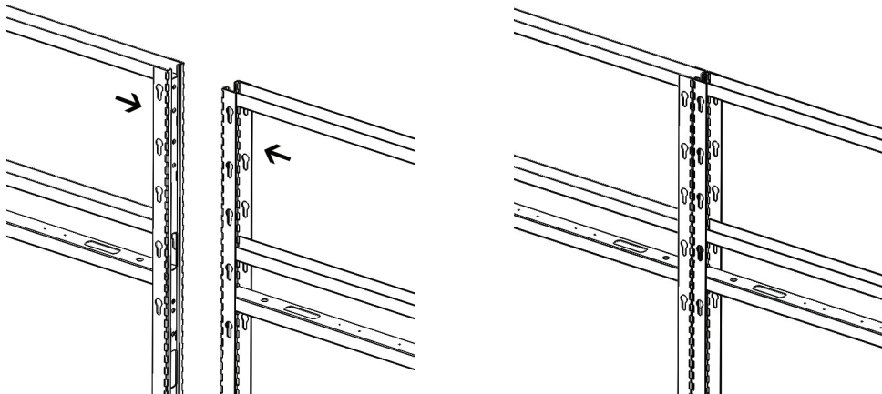
Connection Brakect
