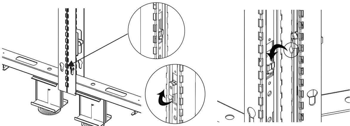
Connection Brakect
